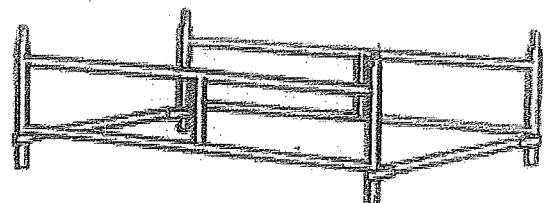
Step 2 (Long Frames) Two frames of equal length placed in ends of anchor bars.
