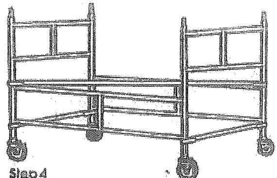
Step 4 Add alternative pairs of frames Add 4 castor wheels
